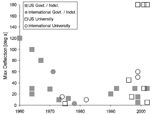
Fig. 15 Overview of air-bearing testbed capabilities: tilt (degrees ±).
